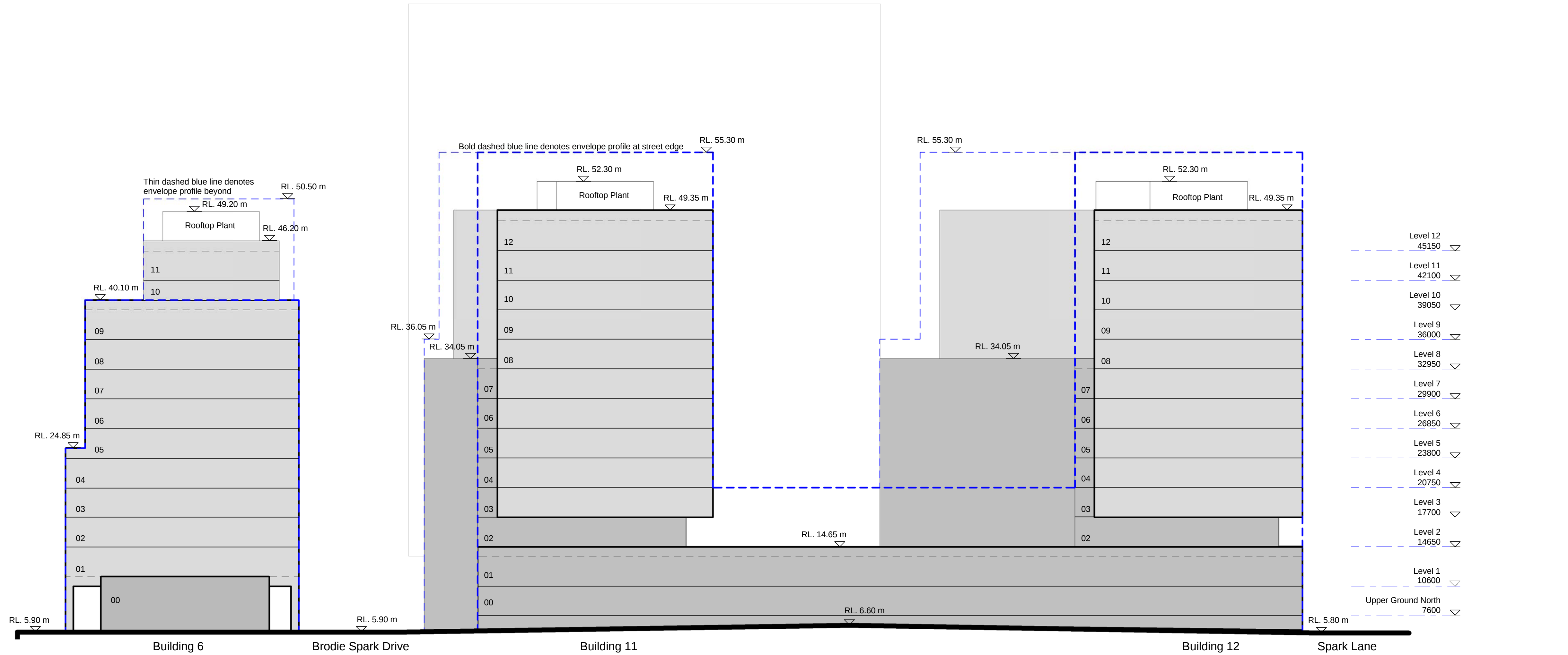
1 Street Elevation - Chisholm Street 7/11/12 1 : 250
